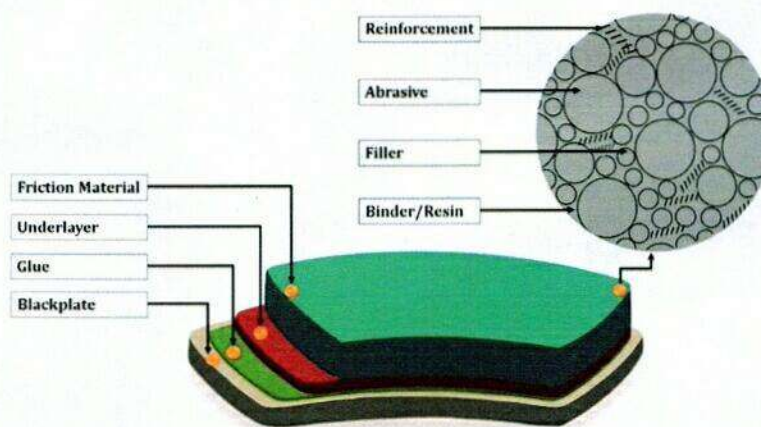
Figure 3. The layers of the brake pad.
