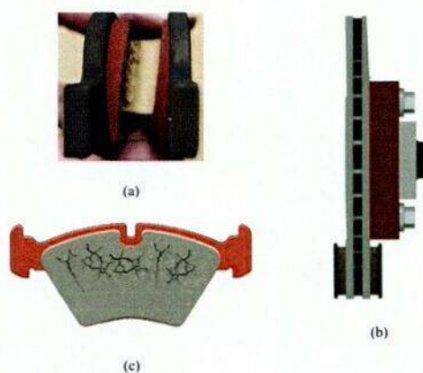
Figure 2. Failure on brake pads caused by excessive thermal loading (a) wears, (b) disc thickness variations, and (c) surface cracking.
