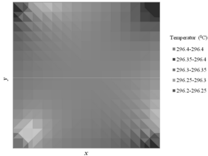
Gambar 2. Distribusi Temperatur
