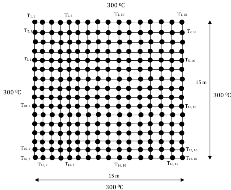
Gambar 1. Distribusi Node
