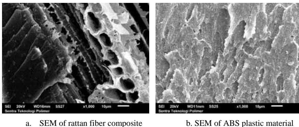
Figure 2 Morphology test using SEM 1000x [1], [2]
